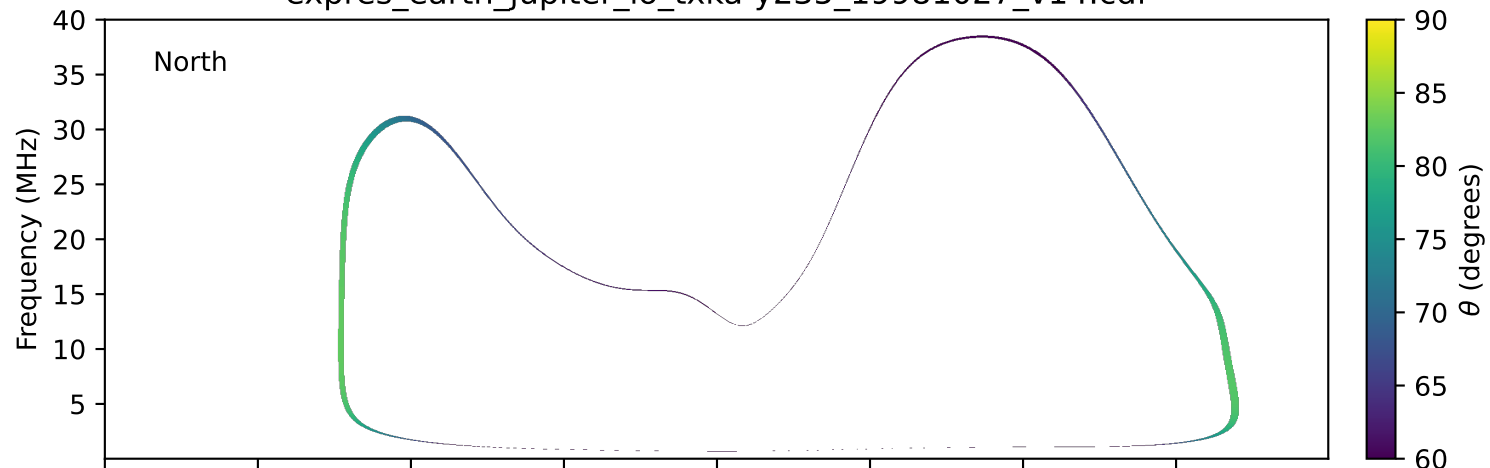
expres_earth_jupiter_io_txka-y235_19981027_v14.cdf
