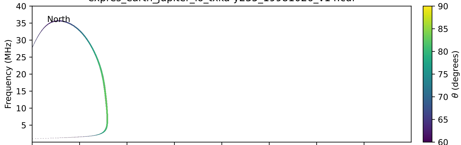
expres_earth_jupiter_io_txka-y235_19981026_v14.cdf
