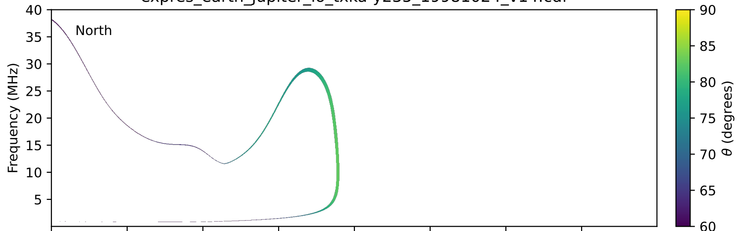
expres_earth_jupiter_io_txka-y235_19981024_v14.cdf
