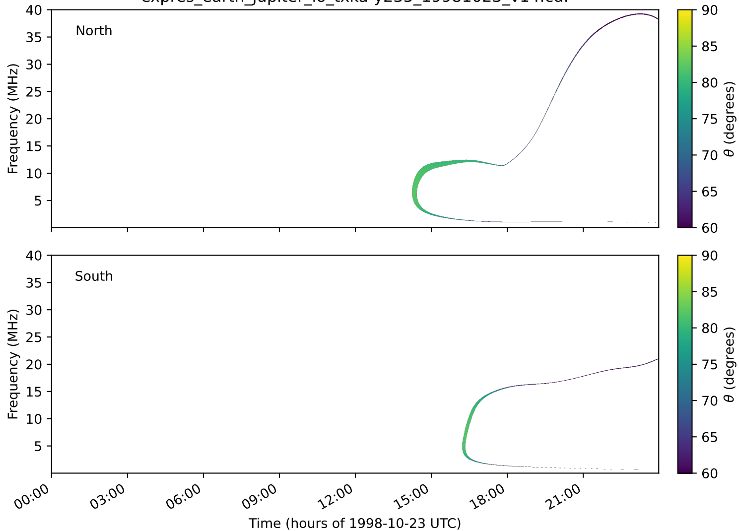
expres_earth_jupiter_io_txka-y235_19981023_v14.cdf
