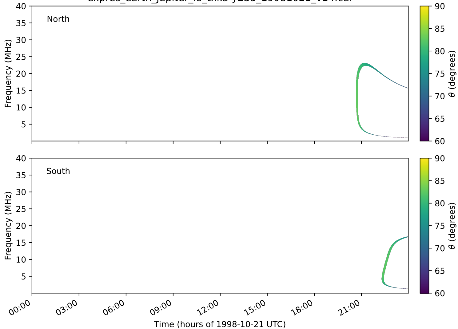
expres_earth_jupiter_io_txka-y235_19981021_v14.cdf
