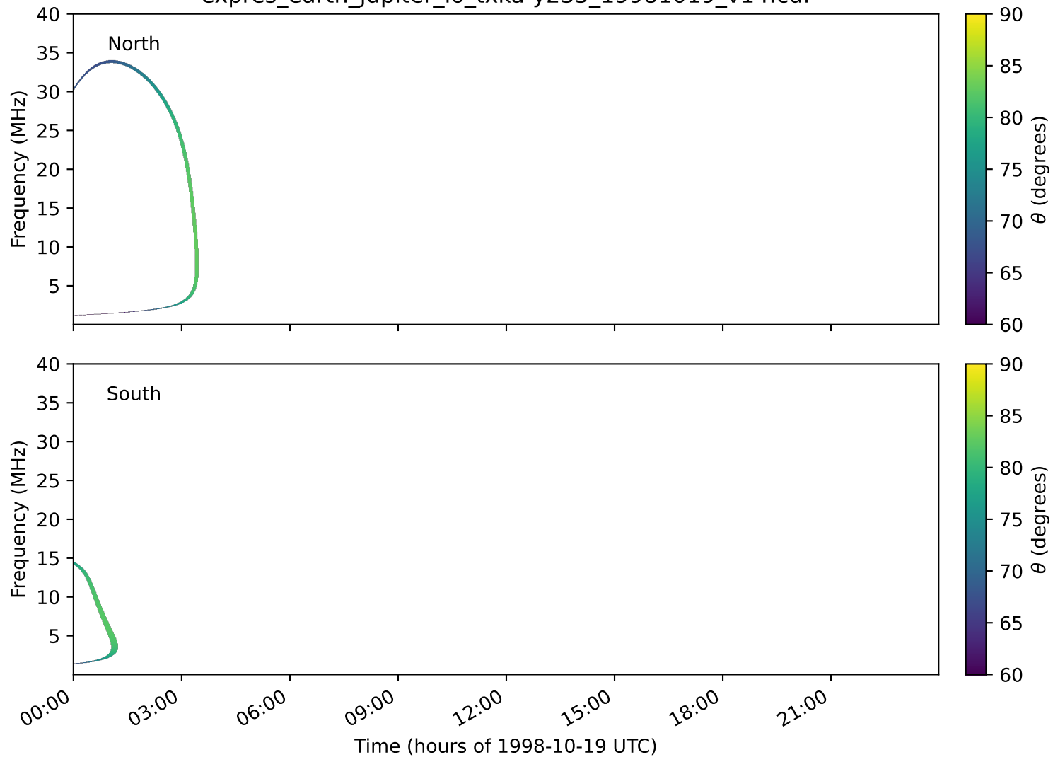
expres_earth_jupiter_io_txka-y235_19981019_v14.cdf
