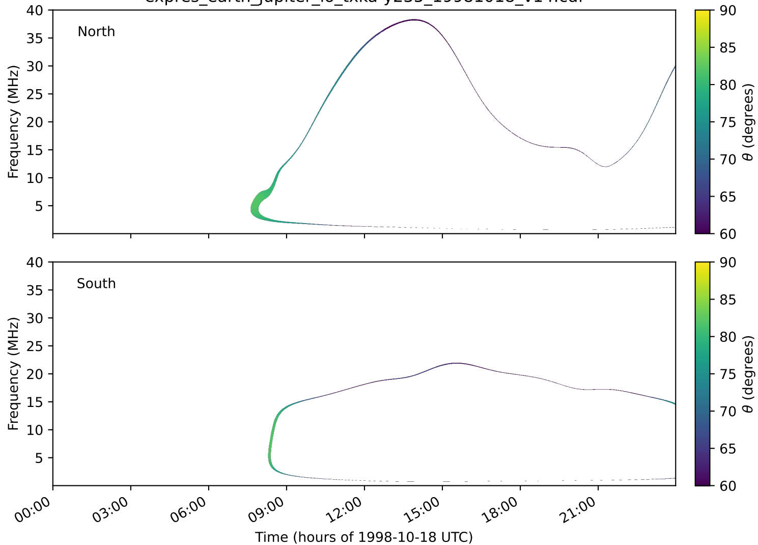
expres_earth_jupiter_io_txka-y235_19981018_v14.cdf
