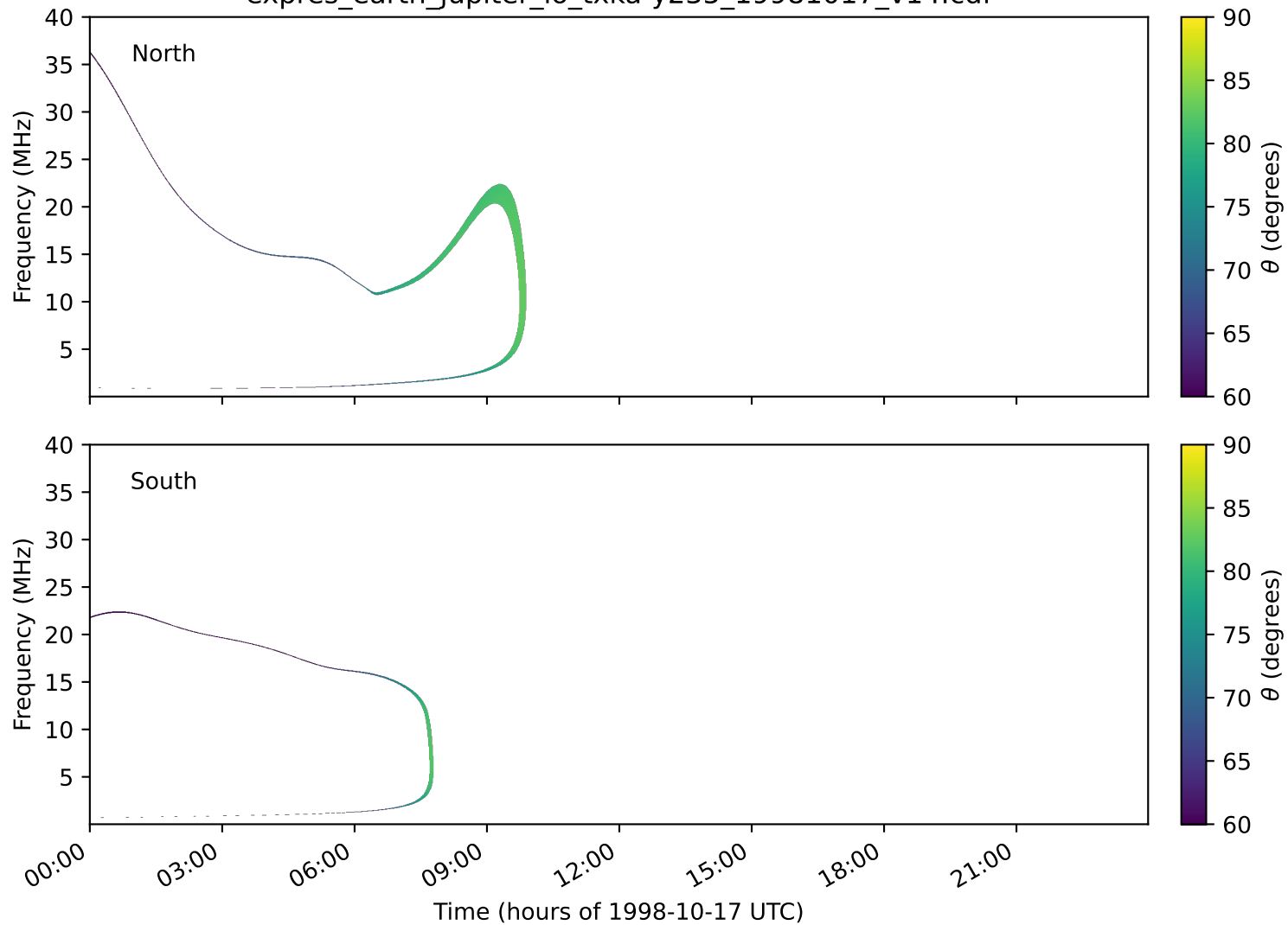
expres_earth_jupiter_io_txka-y235_19981017_v14.cdf
