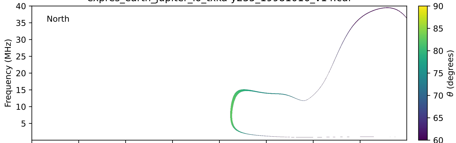
expres_earth_jupiter_io_txka-y235_19981016_v14.cdf
