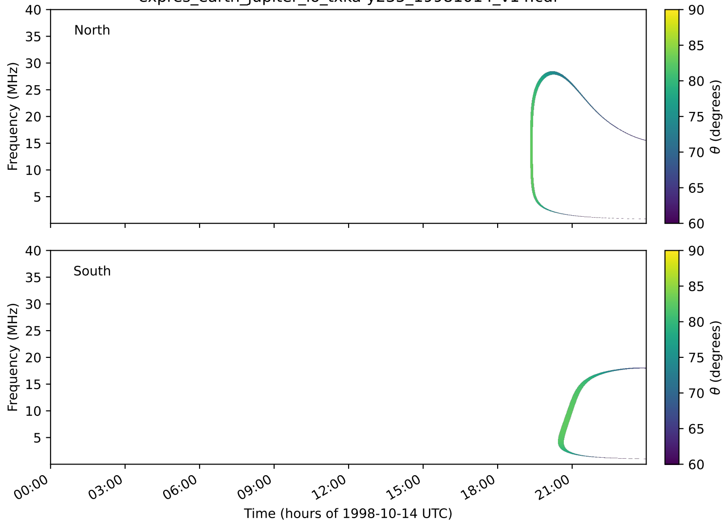
expres_earth_jupiter_io_txka-y235_19981014_v14.cdf
