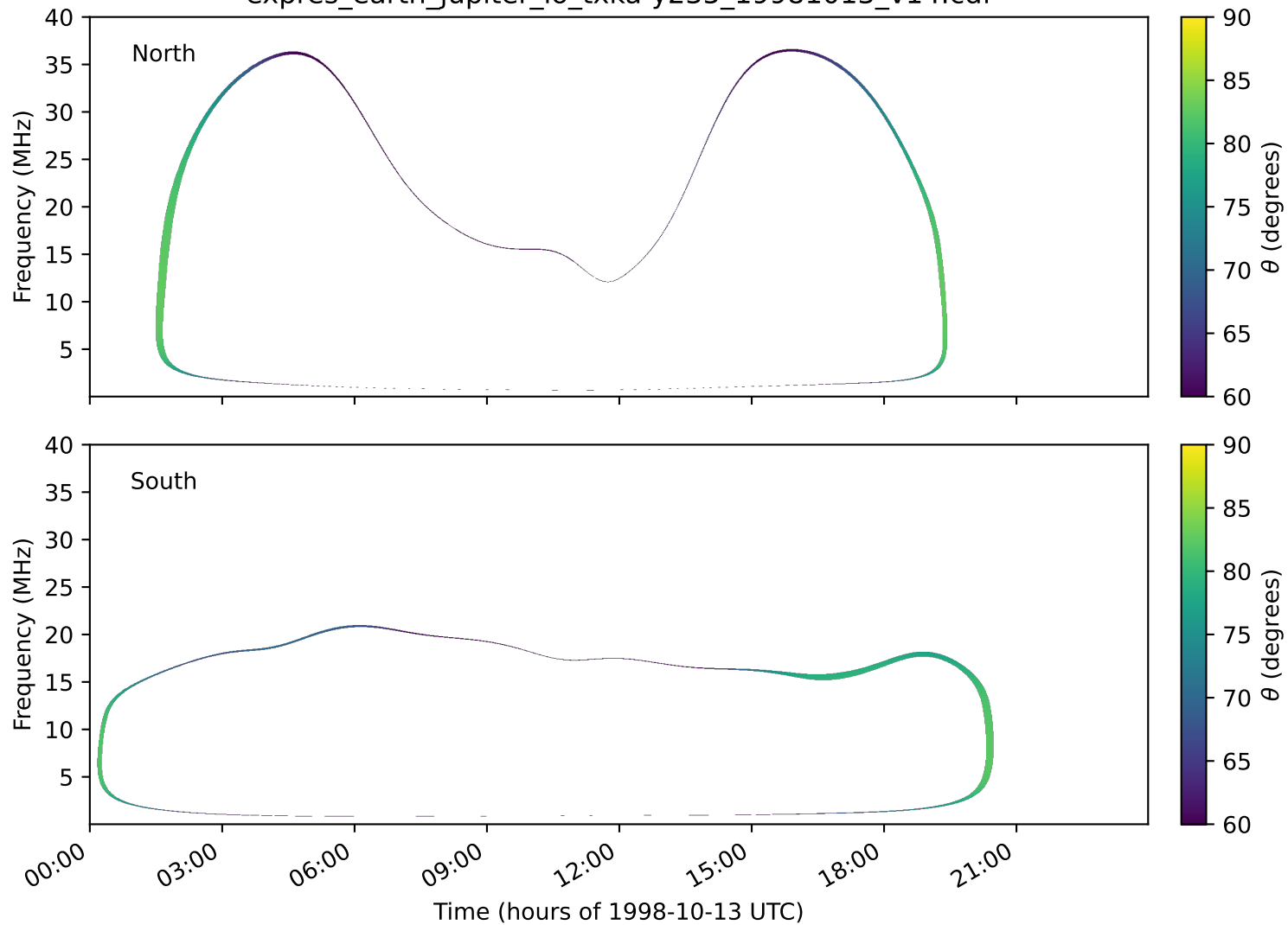
expres_earth_jupiter_io_txka-y235_19981013_v14.cdf
