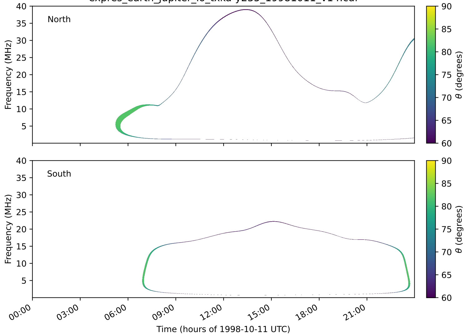
expres_earth_jupiter_io_txka-y235_19981011_v14.cdf
