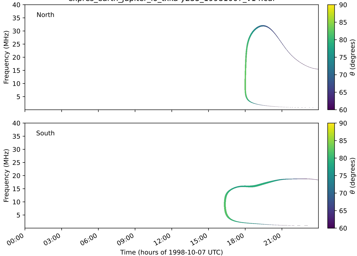
expres_earth_jupiter_io_txka-y235_19981007_v14.cdf
