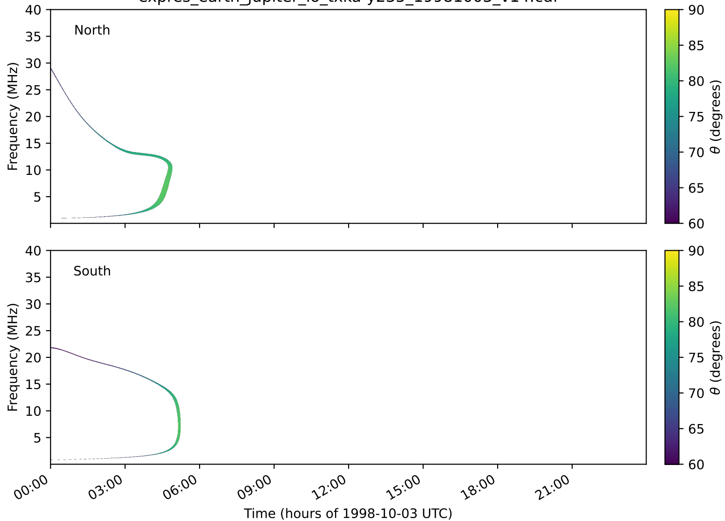
expres_earth_jupiter_io_txka-y235_19981003_v14.cdf
