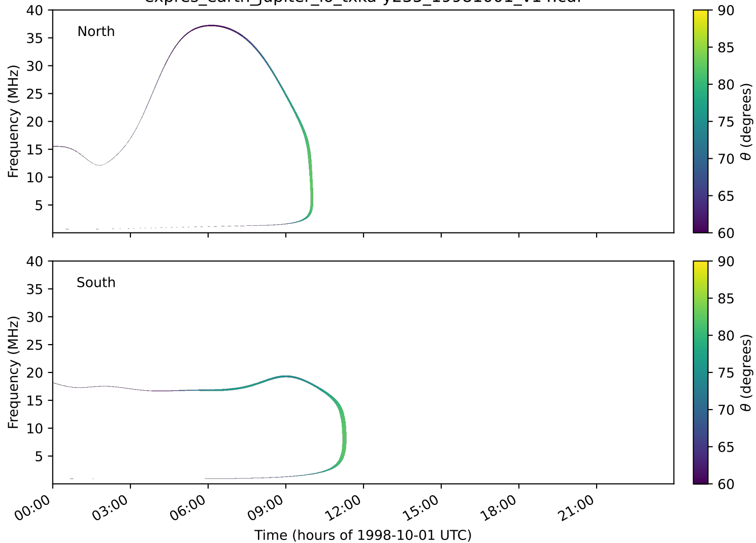
expres_earth_jupiter_io_txka-y235_19981001_v14.cdf
