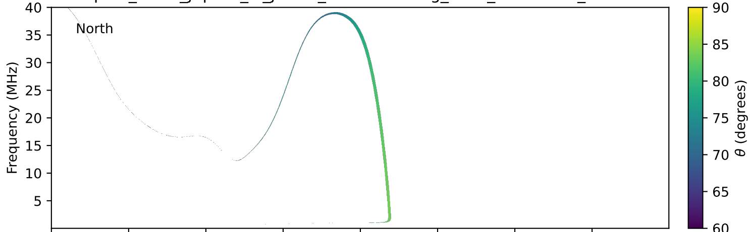
expres_earth_jupiter_io_jrm33_lossc-wid1deg_3kev_19981031_v11.cdf
