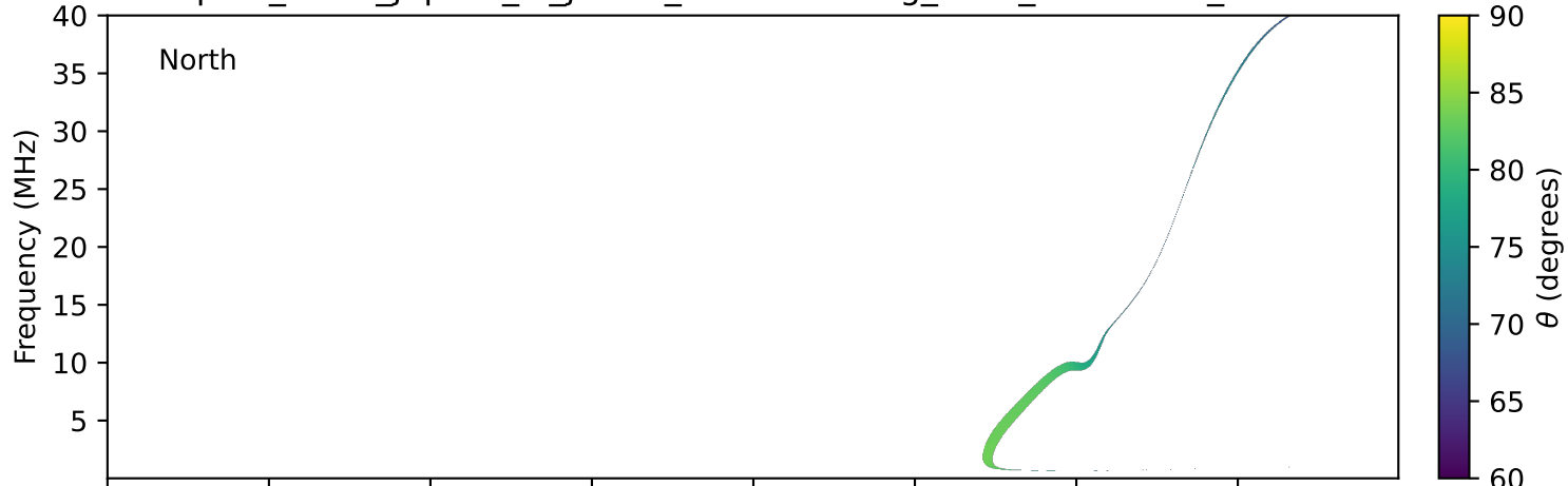
expres_earth_jupiter_io_jrm33_lossc-wid1deg_3kev_19981030_v11.cdf
