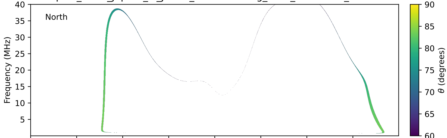
expres_earth_jupiter_io_jrm33_lossc-wid1deg_3kev_19981027_v11.cdf
