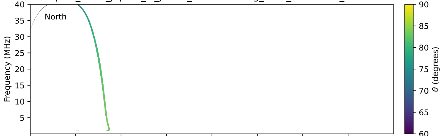
expres_earth_jupiter_io_jrm33_lossc-wid1deg_3kev_19981026_v11.cdf
