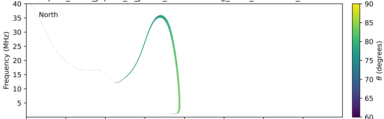
expres_earth_jupiter_io_jrm33_lossc-wid1deg_3kev_19981024_v11.cdf
