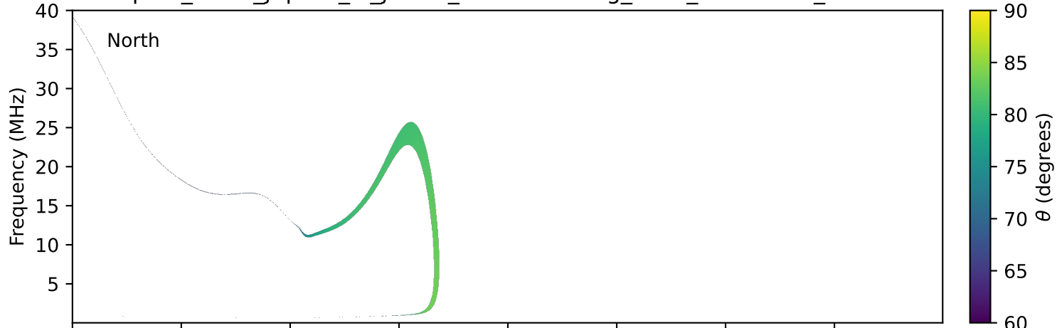
expres_earth_jupiter_io_jrm33_lossc-wid1deg_3kev_19981017_v11.cdf
