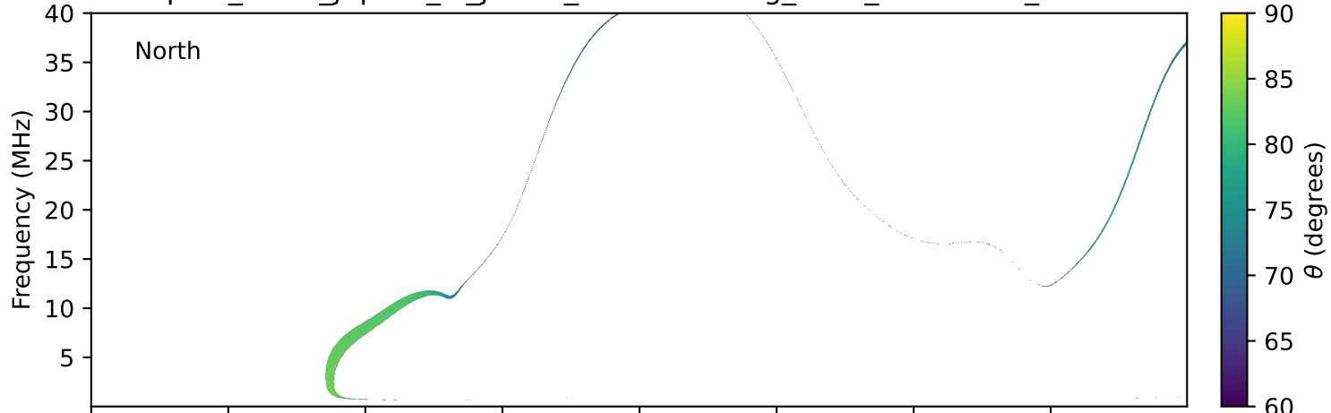
expres_earth_jupiter_io_jrm33_lossc-wid1deg_3kev_19981011_v11.cdf
