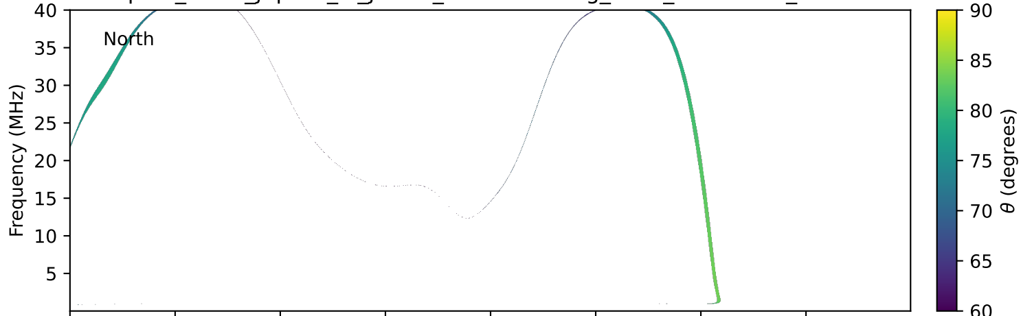
expres_earth_jupiter_io_jrm33_lossc-wid1deg_3kev_19981006_v11.cdf
