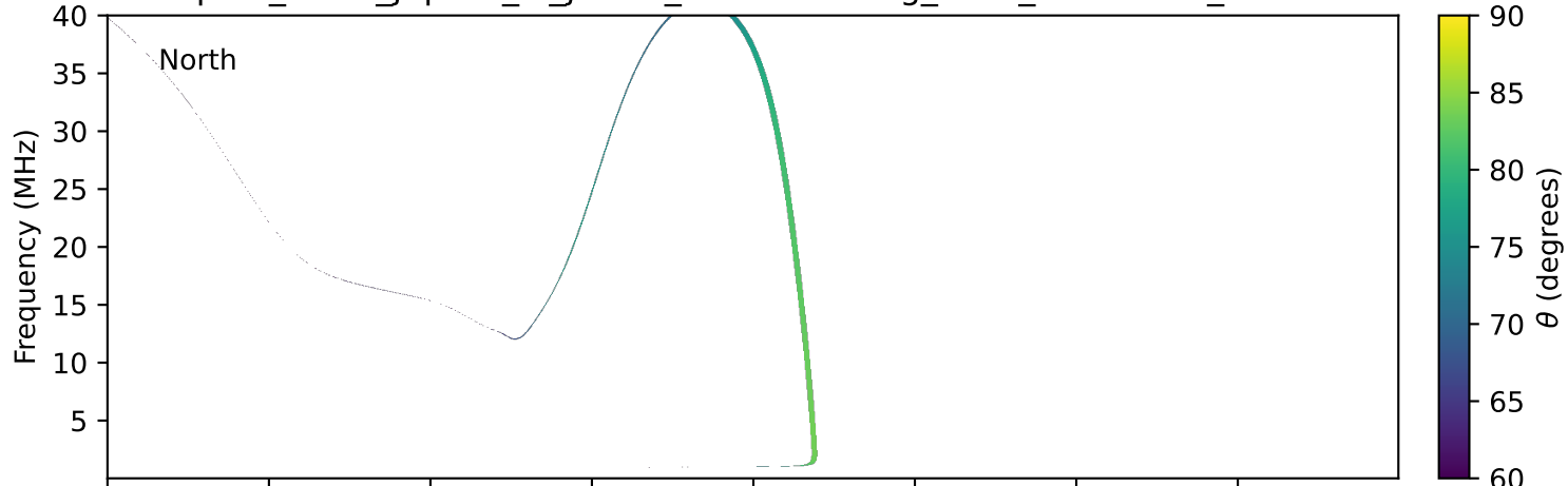
expres_earth_jupiter_io_jrm09_lossc-wid1deg_3kev_19981031_v11.cdf
