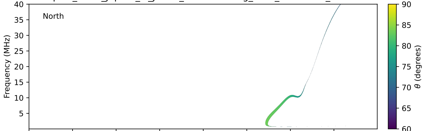
expres_earth_jupiter_io_jrm09_lossc-wid1deg_3kev_19981030_v11.cdf
