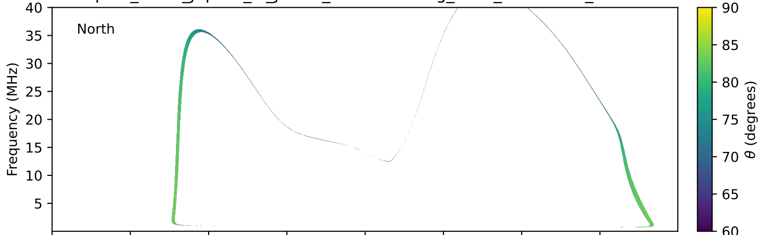
expres_earth_jupiter_io_jrm09_lossc-wid1deg_3kev_19981027_v11.cdf
