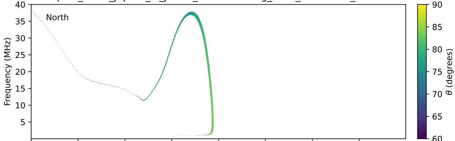
expres_earth_jupiter_io_jrm09_lossc-wid1deg_3kev_19981024_v11.cdf
