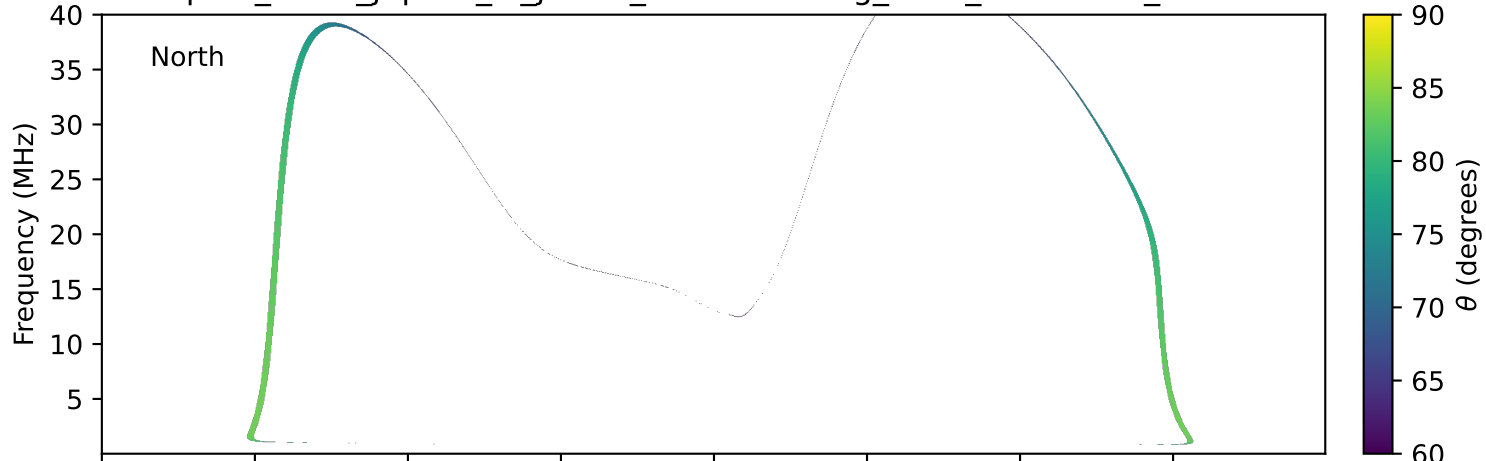
expres_earth_jupiter_io_jrm09_lossc-wid1deg_3kev_19981020_v11.cdf
