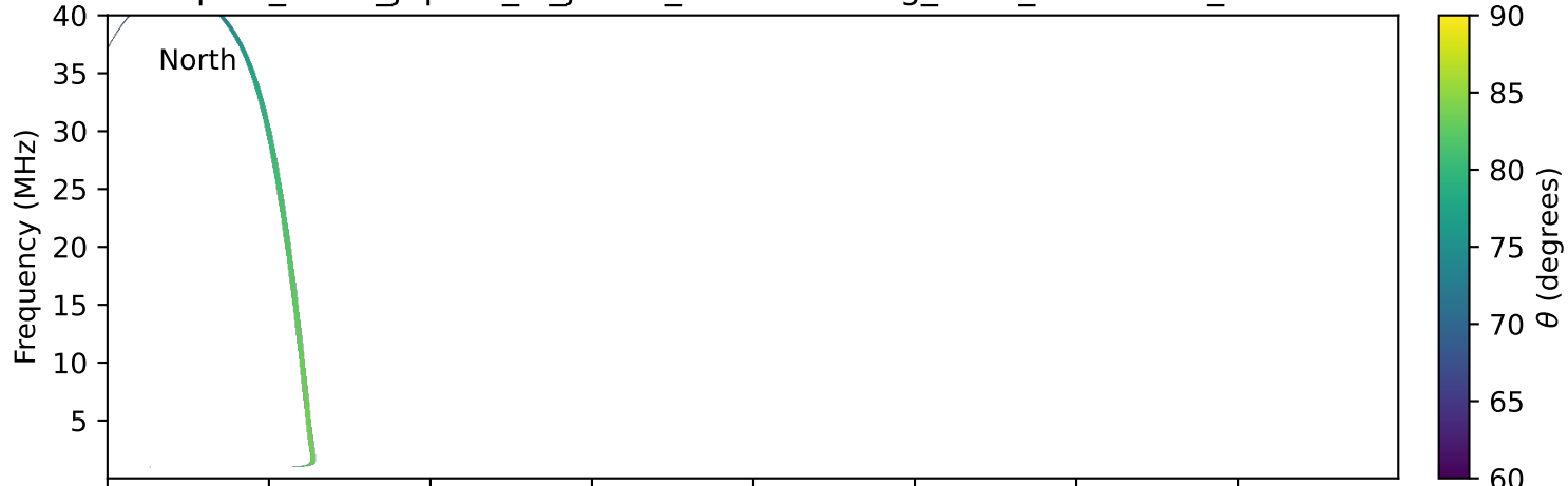
expres_earth_jupiter_io_jrm09_lossc-wid1deg_3kev_19981019_v11.cdf
