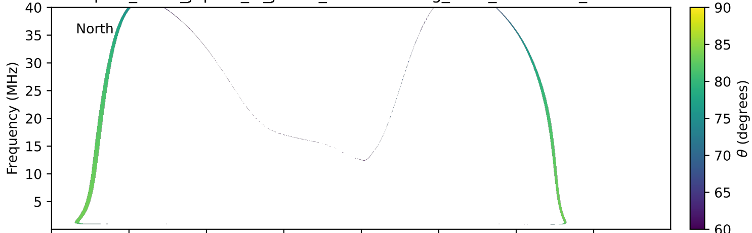
expres_earth_jupiter_io_jrm09_lossc-wid1deg_3kev_19981013_v11.cdf
