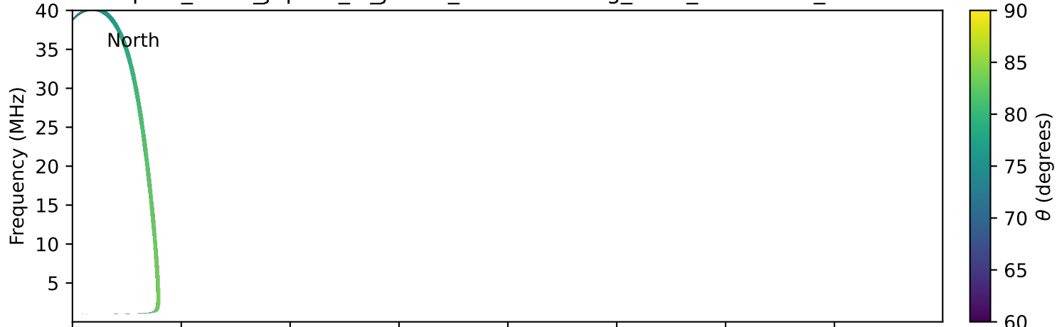
expres_earth_jupiter_io_jrm09_lossc-wid1deg_3kev_19981012_v11.cdf
