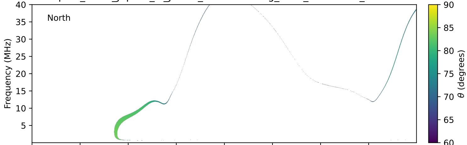
expres_earth_jupiter_io_jrm09_lossc-wid1deg_3kev_19981011_v11.cdf
