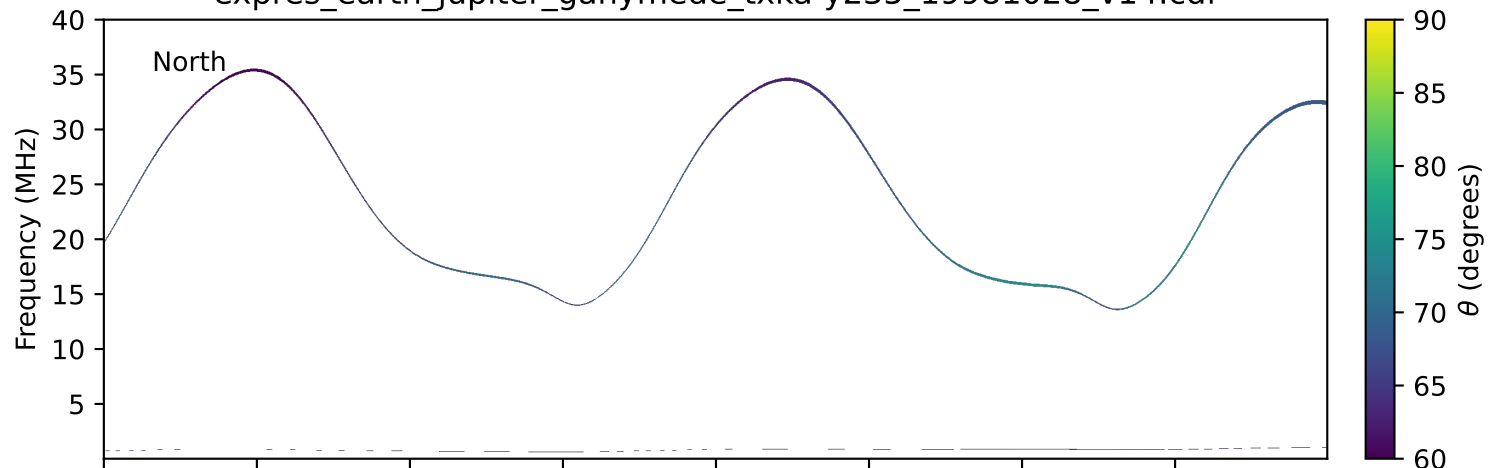
expres_earth_jupiter_ganymede_txka-y235_19981028_v14.cdf
