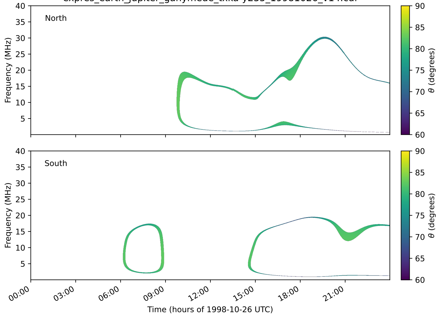
expres_earth_jupiter_ganymede_txka-y235_19981026_v14.cdf
