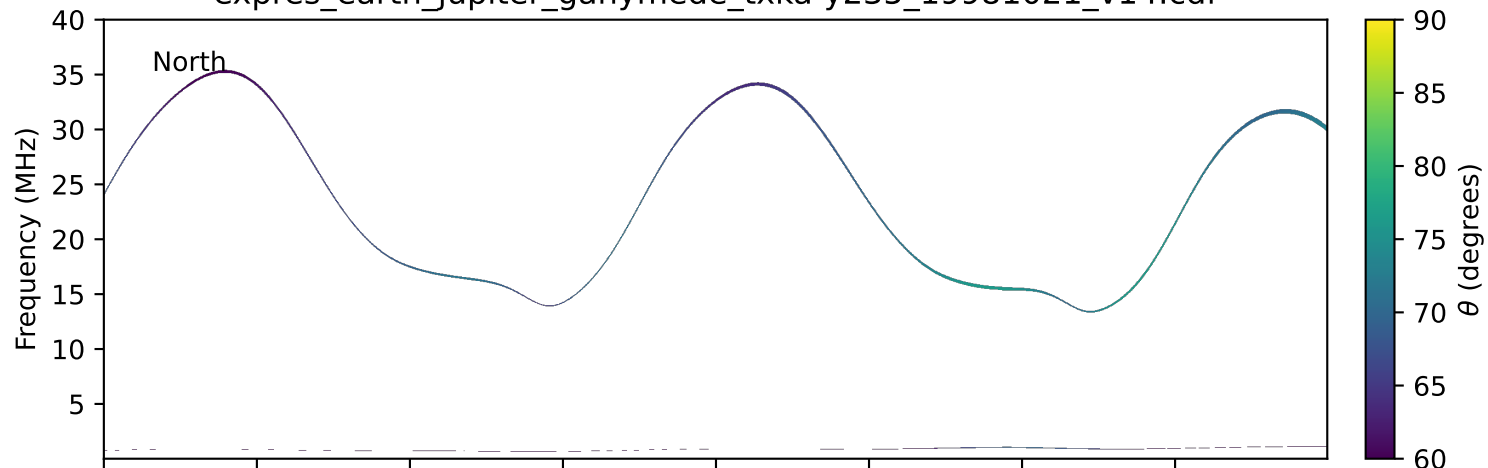
expres_earth_jupiter_ganymede_txka-y235_19981021_v14.cdf
