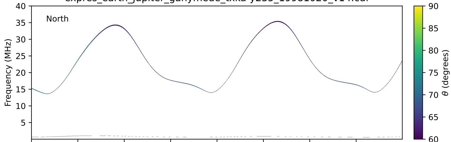
expres_earth_jupiter_ganymede_txka-y235_19981020_v14.cdf
