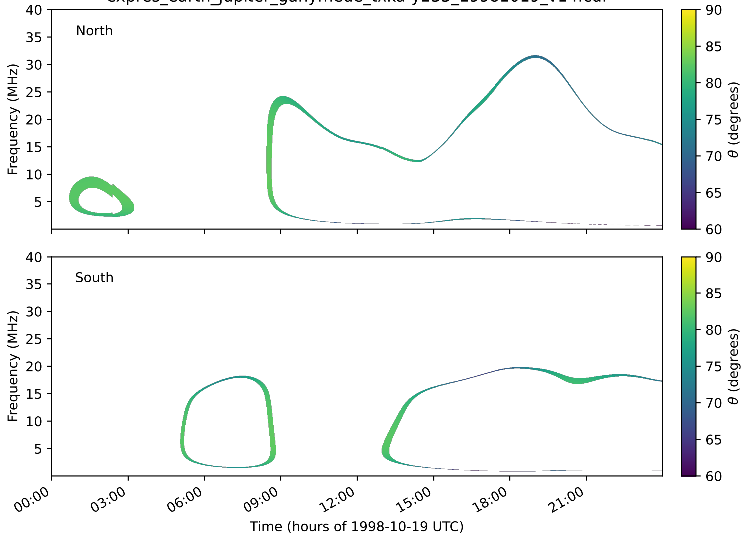
expres_earth_jupiter_ganymede_txka-y235_19981019_v14.cdf
