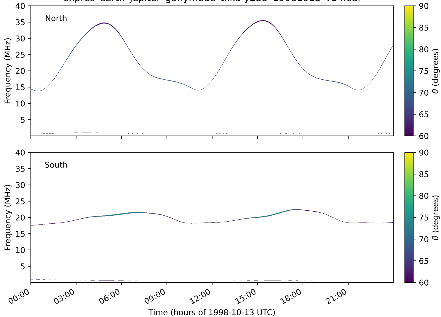
expres_earth_jupiter_ganymede_txka-y235_19981013_v14.cdf
