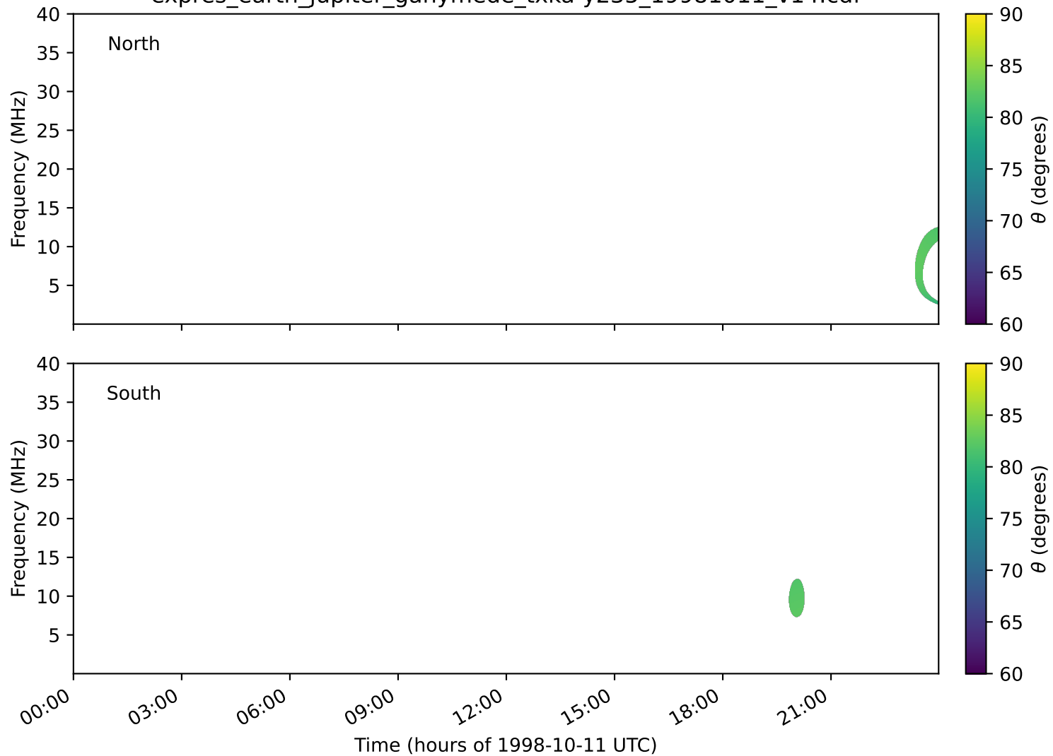
expres_earth_jupiter_ganymede_txka-y235_19981011_v14.cdf
