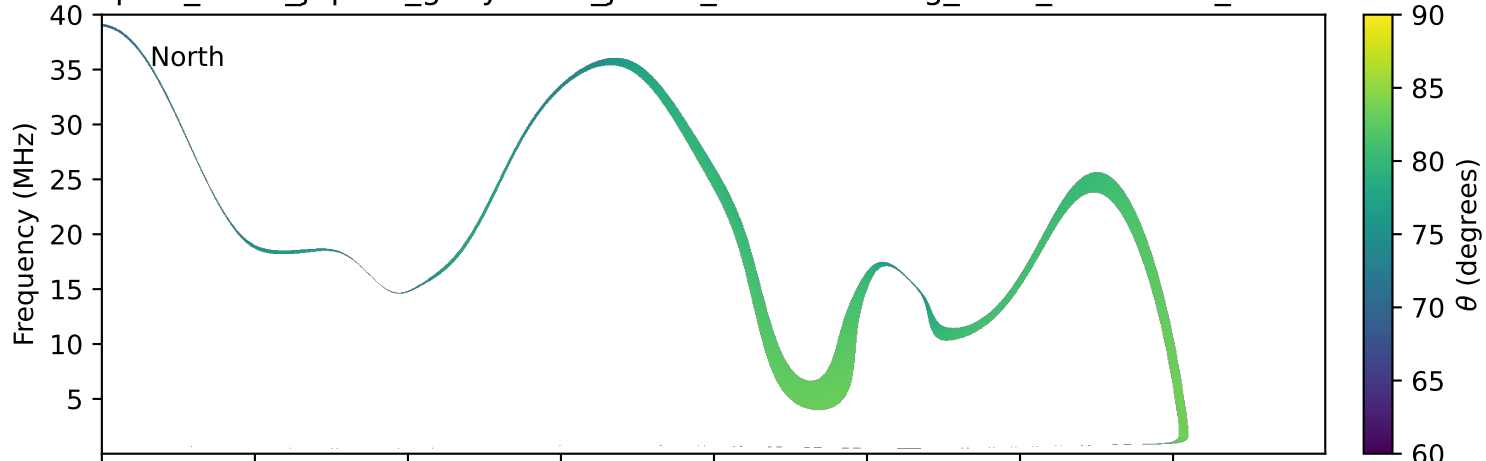
expres_earth_jupiter_ganymede_jrm33_lossc-wid1deg_3kev_19981029_v11.cdf
