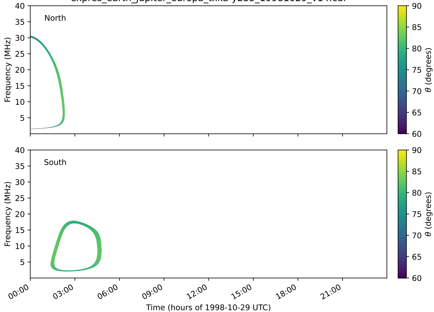
expres_earth_jupiter_europa_txka-y235_19981029_v14.cdf
