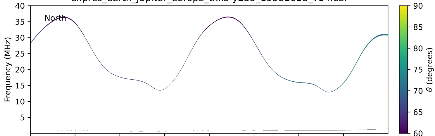
expres_earth_jupiter_europa_txka-y235_19981028_v14.cdf
