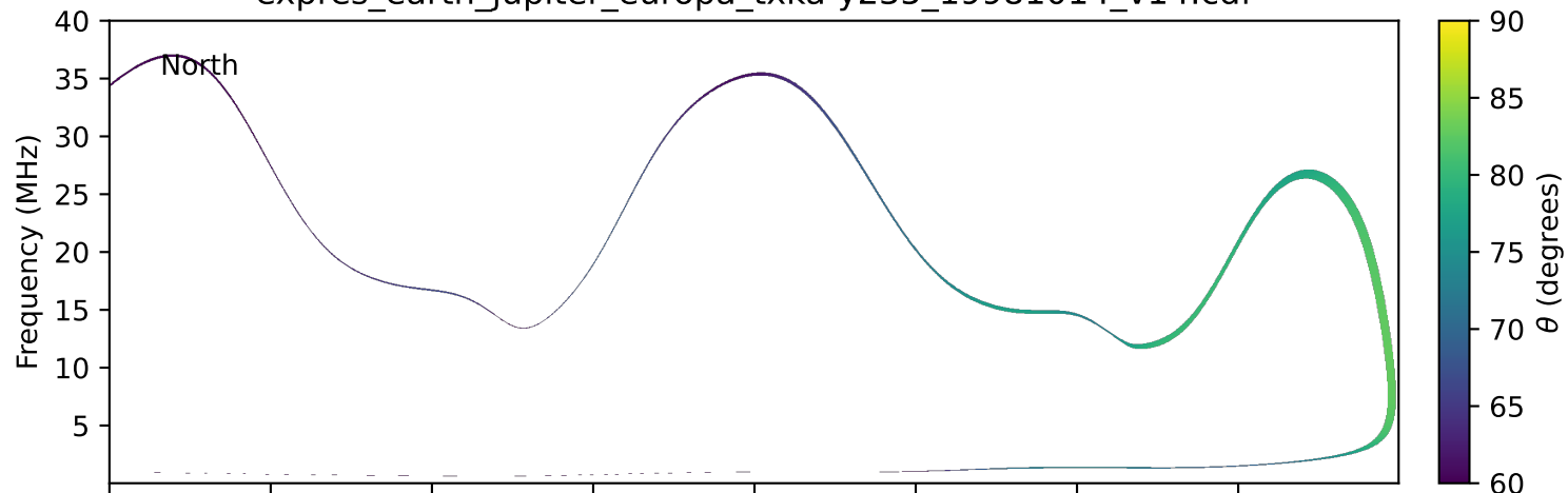
expres_earth_jupiter_europa_txka-y235_19981014_v14.cdf
