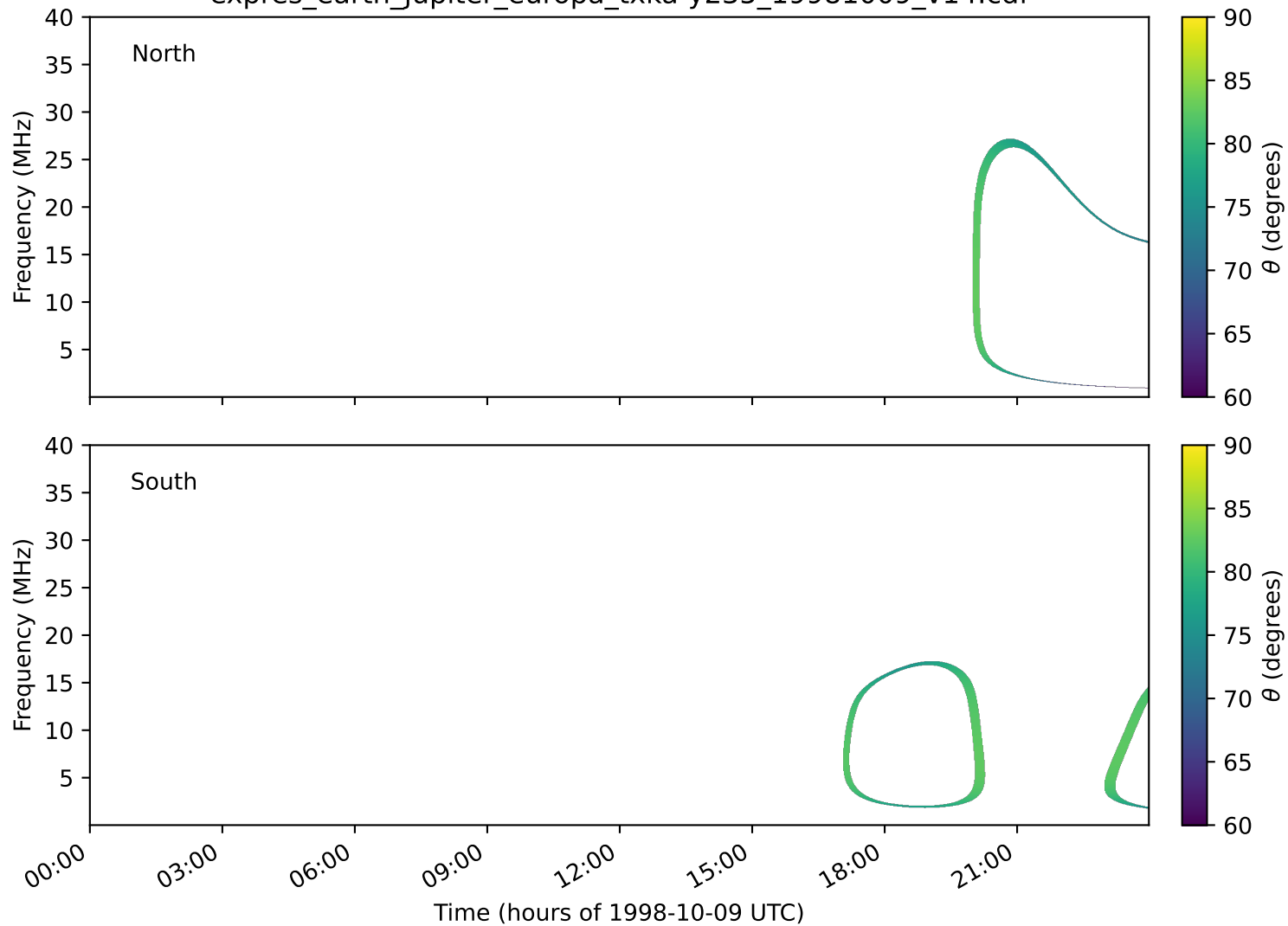
expres_earth_jupiter_europa_txka-y235_19981009_v14.cdf
