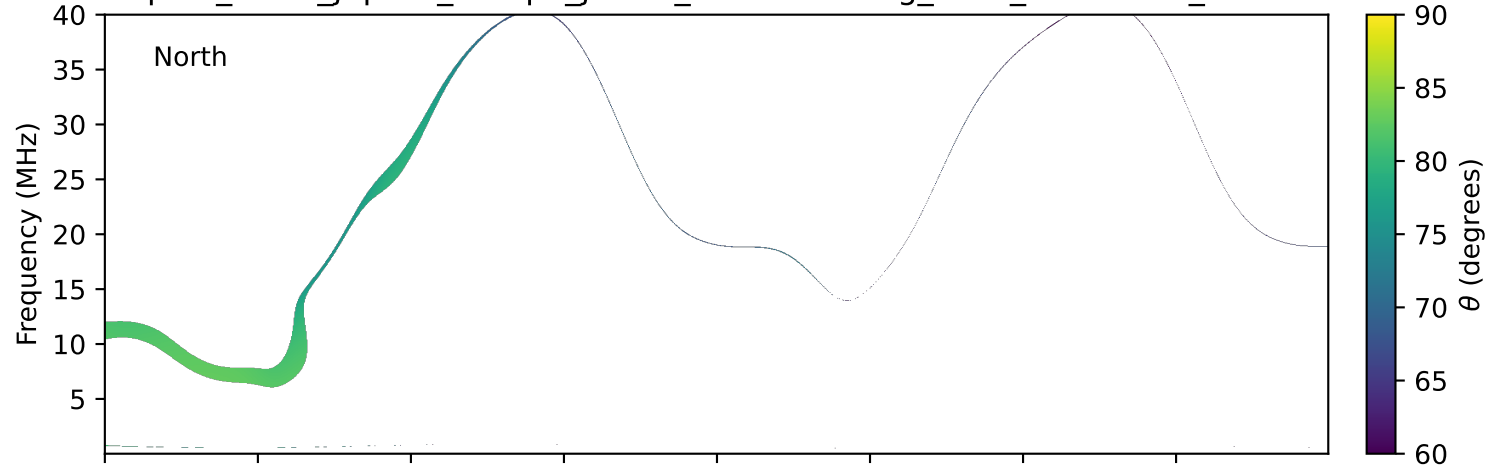
expres_earth_jupiter_europa_jrm33_lossc-wid1deg_3kev_19981024_v11.cdf
