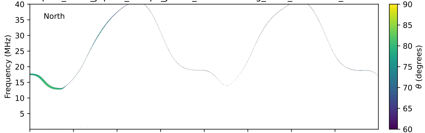
expres_earth_jupiter_europa_jrm33_lossc-wid1deg_3kev_19981010_v11.cdf
