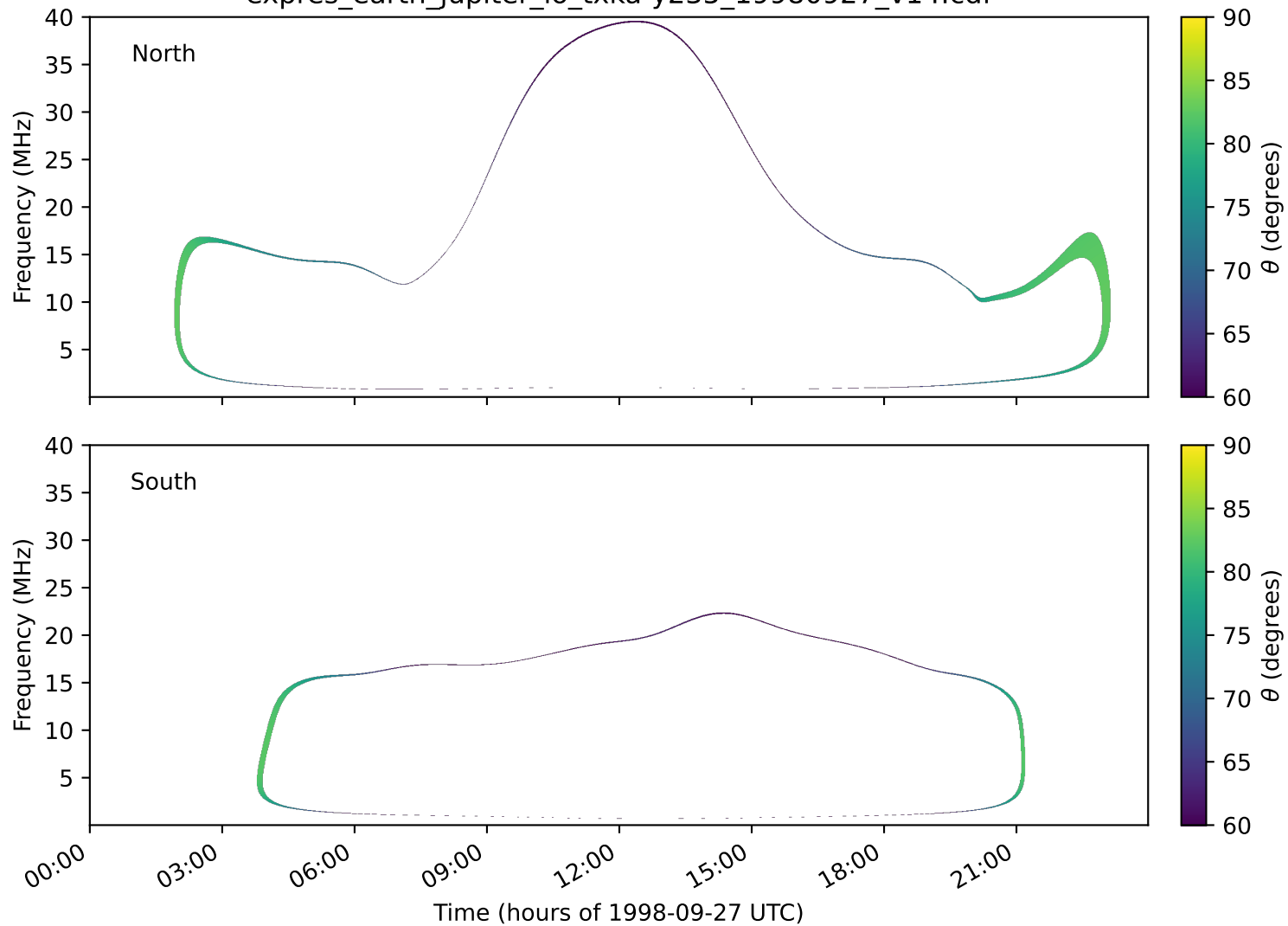
expres_earth_jupiter_io_txka-y235_19980927_v14.cdf
