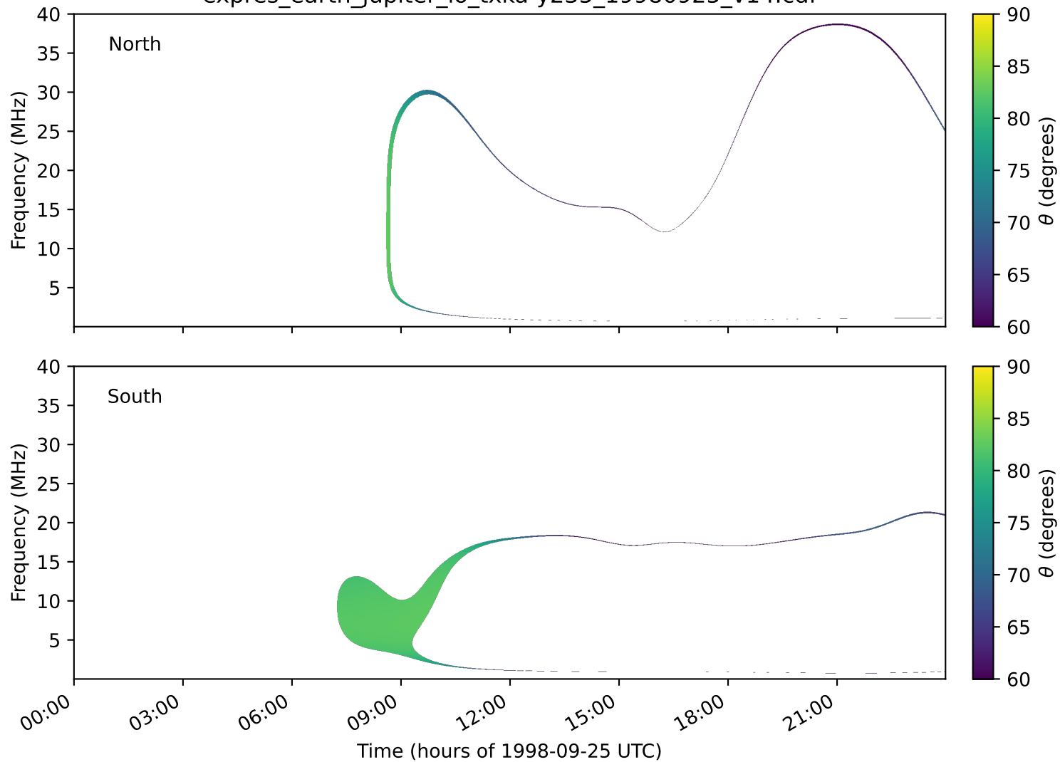
expres_earth_jupiter_io_txka-y235_19980925_v14.cdf
