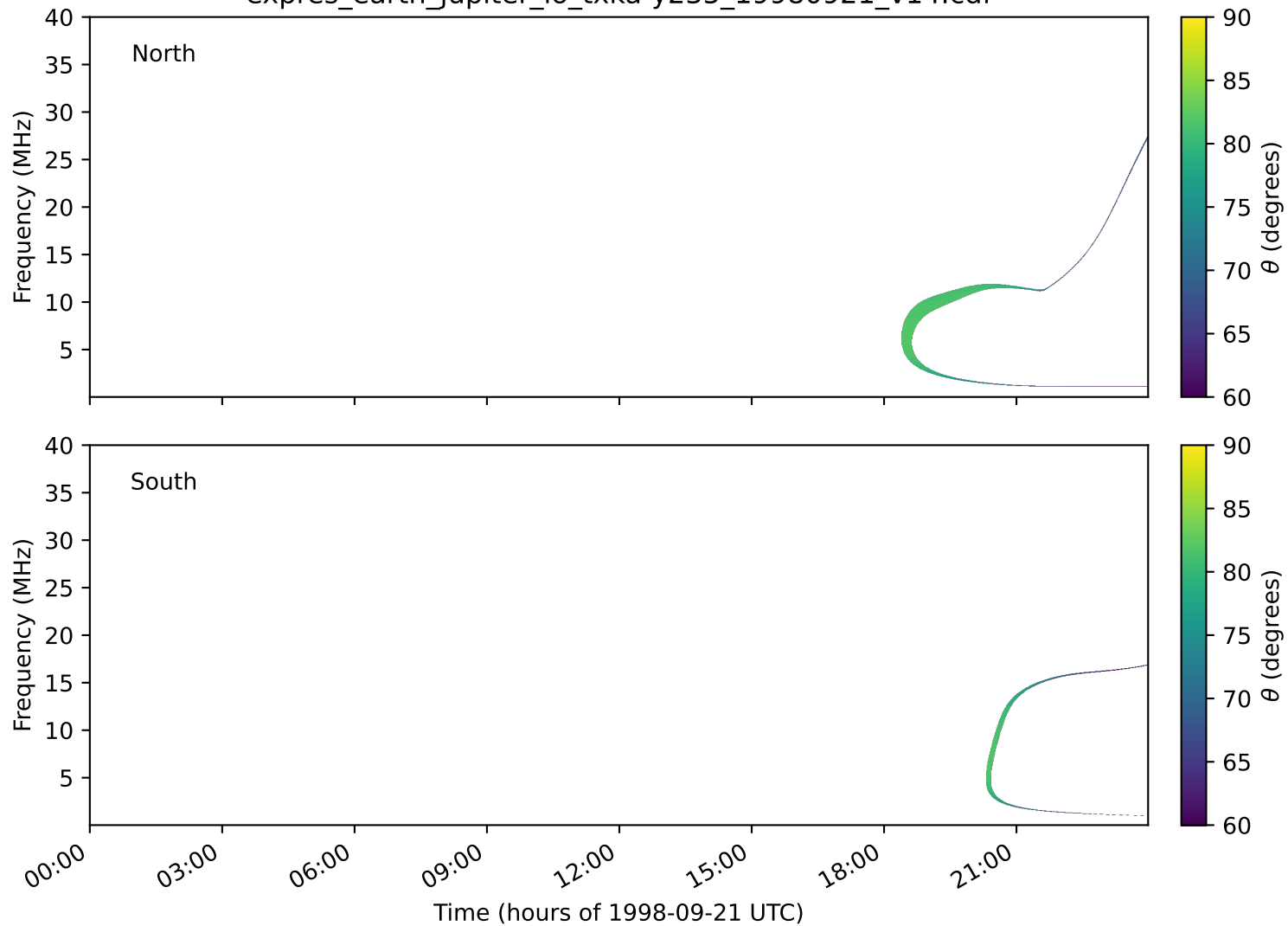
expres_earth_jupiter_io_txka-y235_19980921_v14.cdf
