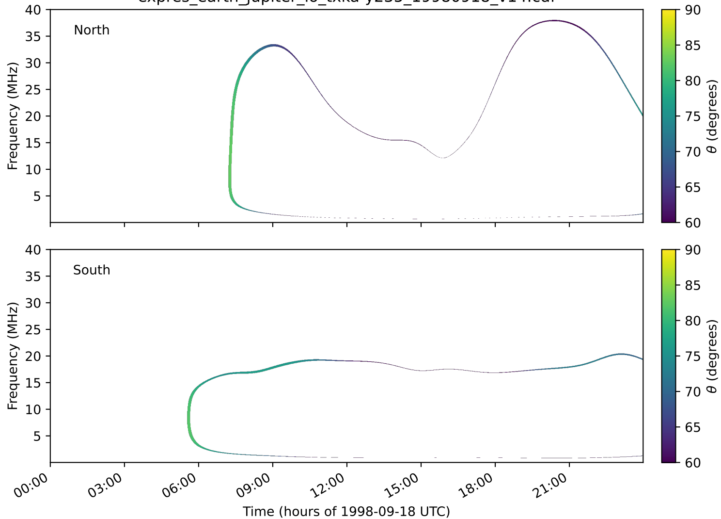
expres_earth_jupiter_io_txka-y235_19980918_v14.cdf
